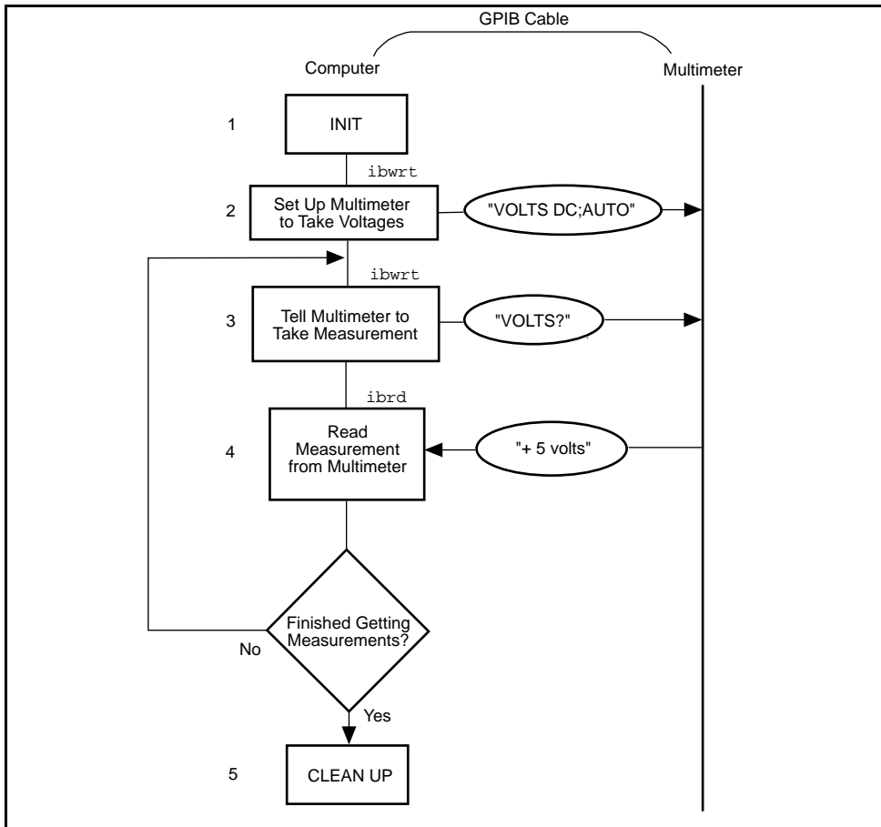
Figure 2-1. Program Flowchart for Example 1
